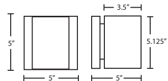
1SW-TITO07-SN 5" L x 5.25" H x 5" D
